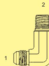
BJ-2501-L - 90°
