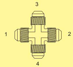
BF-2650-F - Cross
