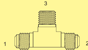
BF-2601 - Tee
