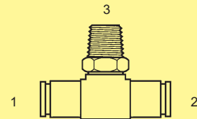
BPC-2601-S - Tee
