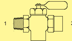
BV-402P-UL - Str. (Marine) (1) Male Pipe (2) Fem. Pipe
