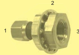
BAB-N-2405-BH - Str. (1) Air Brake (2) Bulkhead (3) Fem. Pipe
