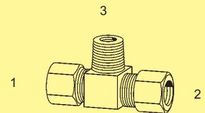
BC-SA-2601 - Tee
