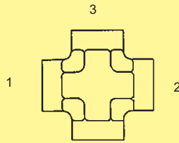
BP-5652-F - Cross
