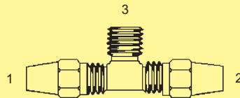
BC-L-2601 - Tee (1) (2) Compression (3) Male Pipe
